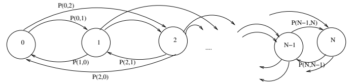
Fig. 2. System state transition diagram in reservation-based access protocol with a fixed number of access slots per frame
